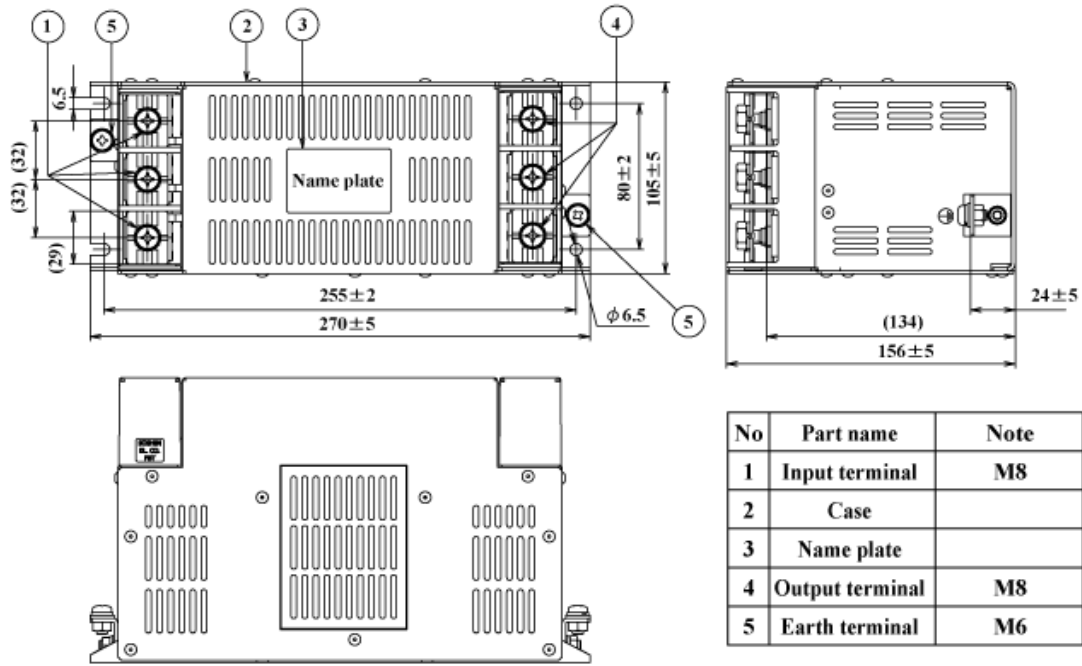
fig.4 (150A, 180A)
