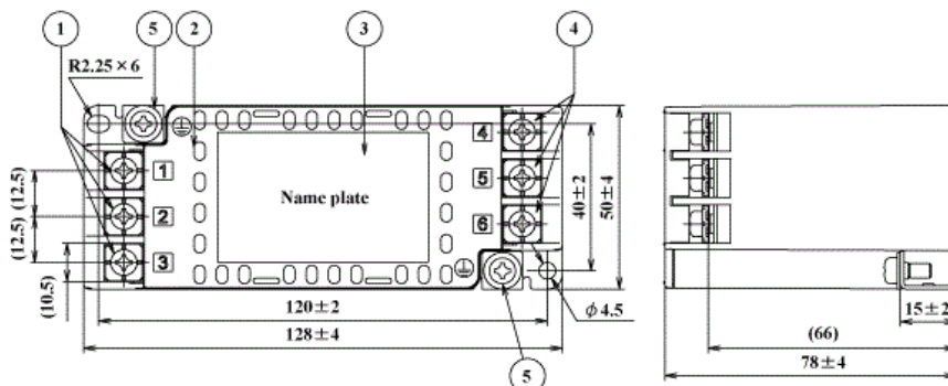
fig.1 (10-30A)
