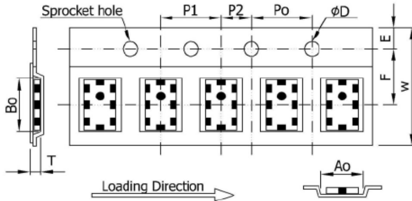
Black conductive Tape specifications (unit :mm)
